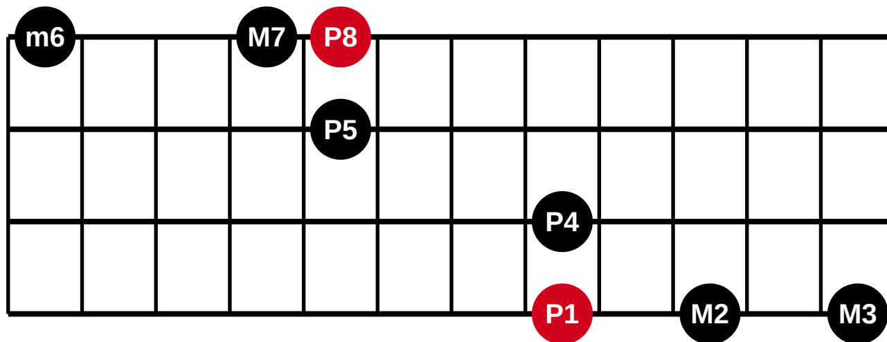
4 strings - 12 frets - fingering 35 of 35
